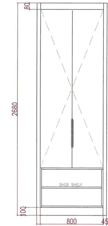
45 GUEST ROOM WARDROBE-2- FRONT VIEW
