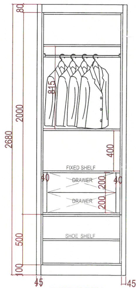
GUEST ROOM WARDROBE-2- INNER VIEW
