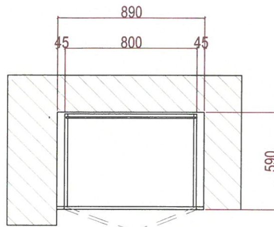
GUEST ROOM 2 WARDROBE-2- LAYOUT
